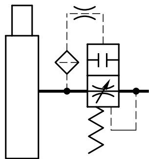
HYDRAULIC SCHEMA
