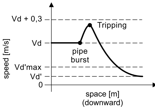
WORKING DIAGRAM
