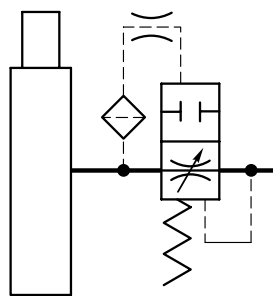
HYDRAULIC SCHEMA
