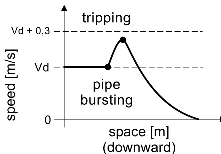
WORKING DIAGRAM
