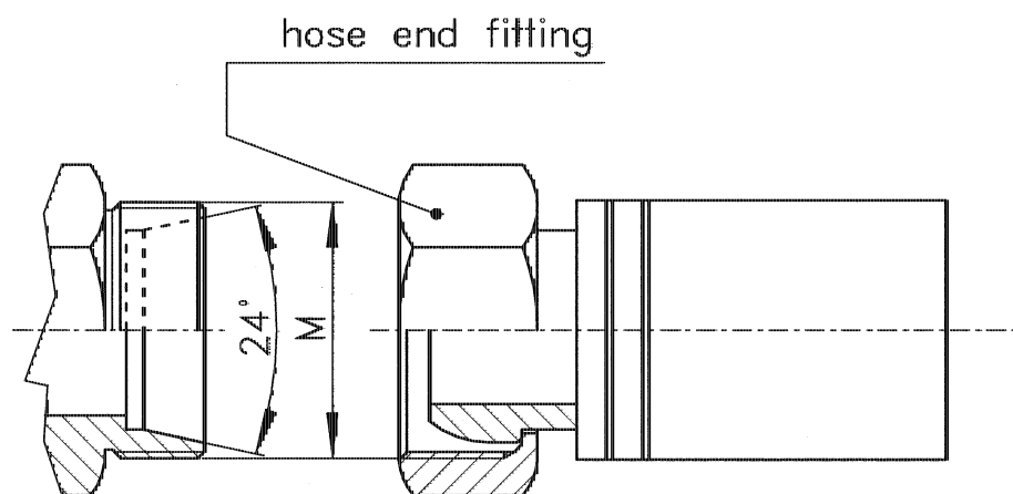
HOSE COUPLING
