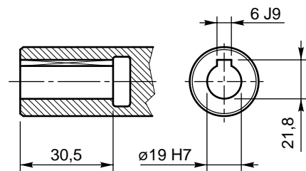
SHAFT DETAIL
