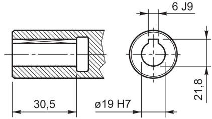
SHAFT DETAIL
