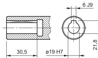
SHAFT DETAIL
