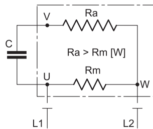
WIRING DIAGRAM
